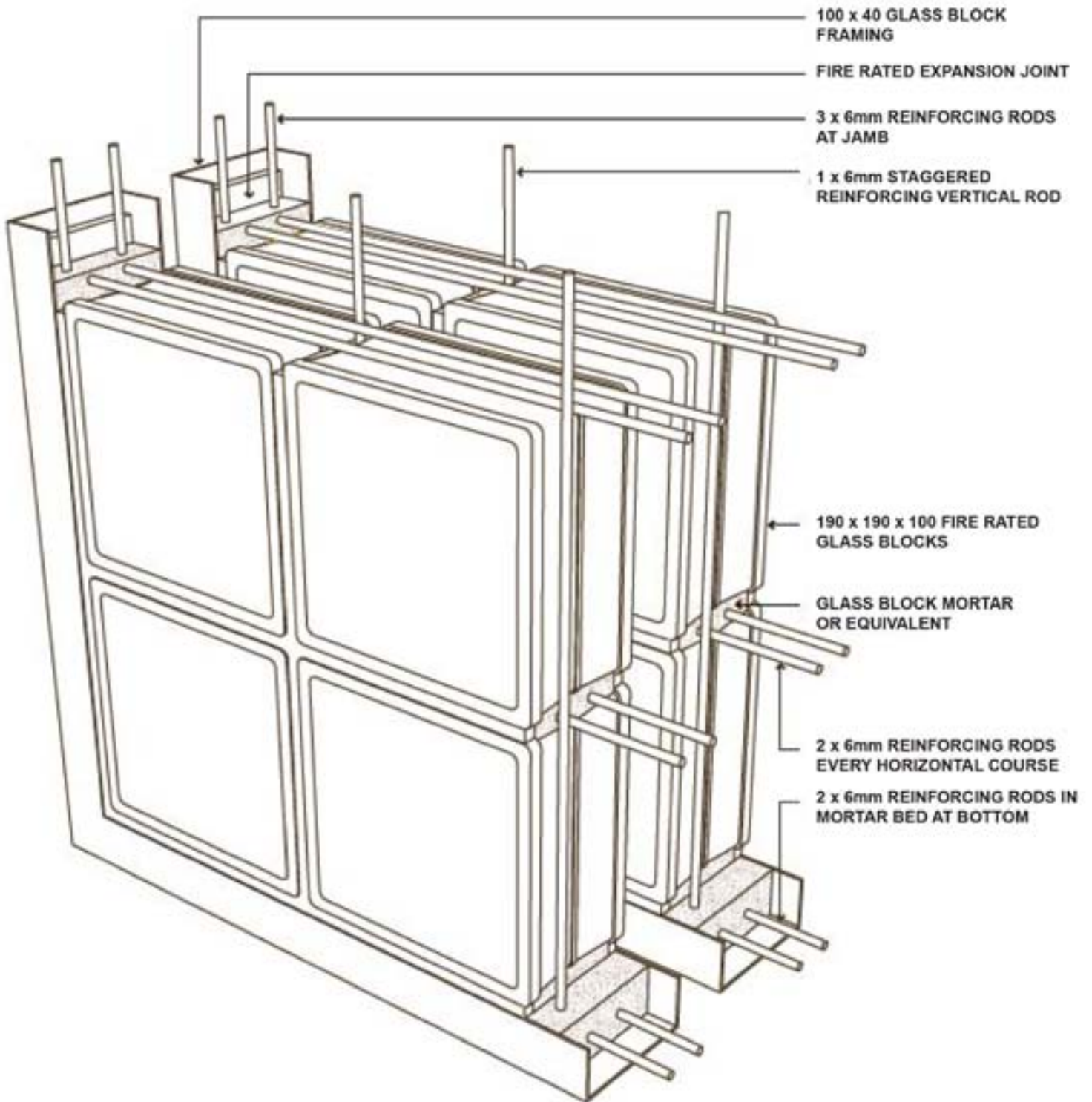
DWG13 : FRL -/120/- Fire Rated Installation
