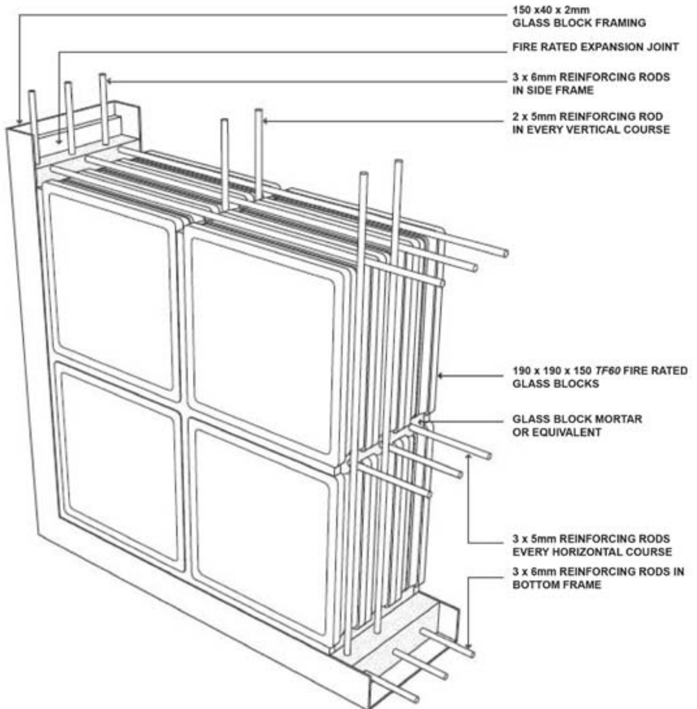
DWG17 : FRL -/90/60 Fire Rated Installation
