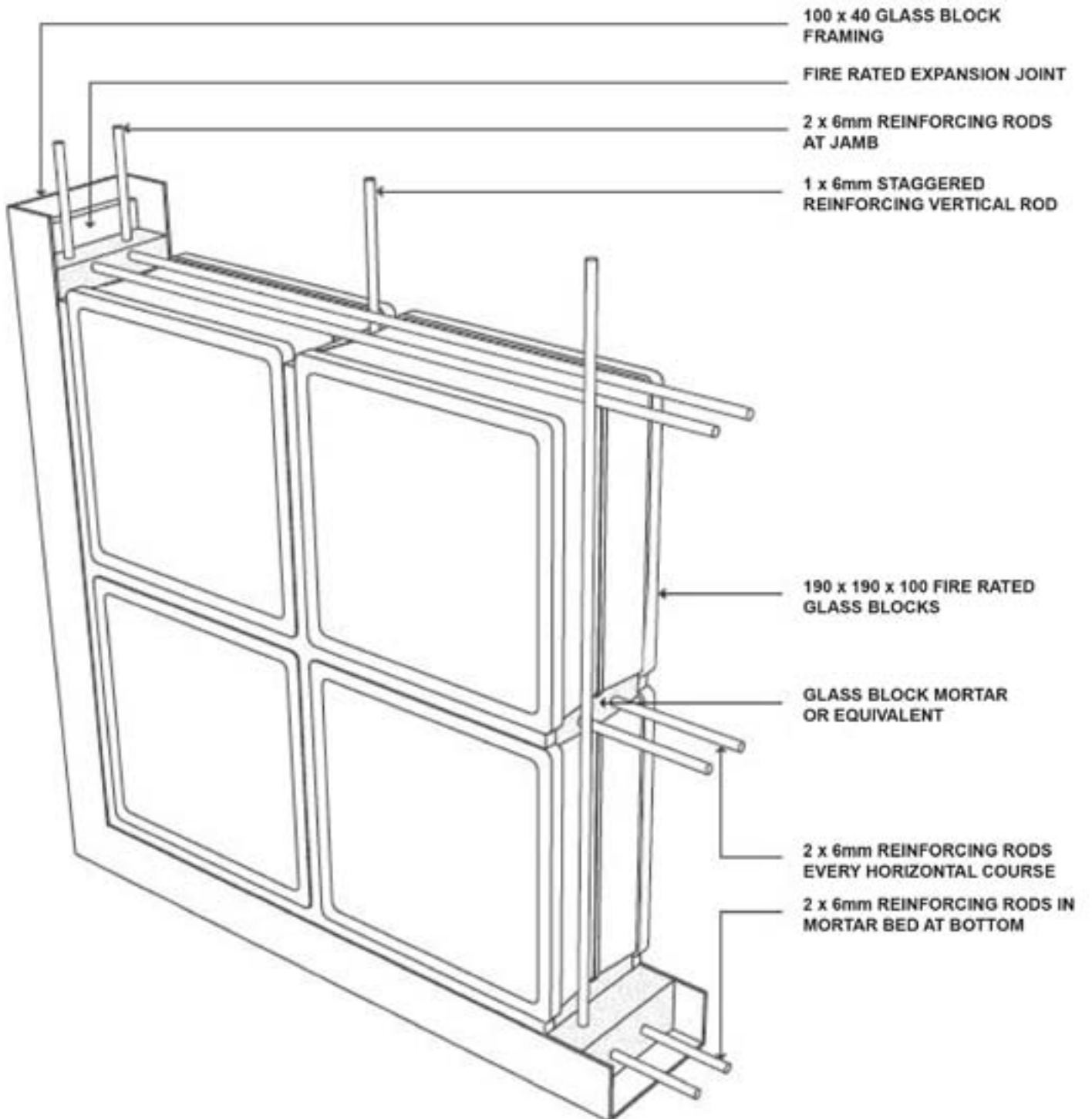
DWG02 : FRL -/90/- Fire Rated Installation
